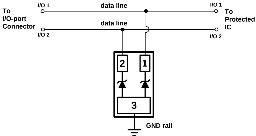
Fig. 1 Data lines connection of AZ5213-02F.
