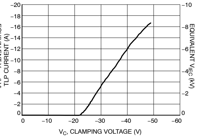
Figure 10. Typical Negative TLP IV Curve
