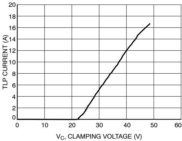
Figure 9. Typical Positive TLP IV Curve
