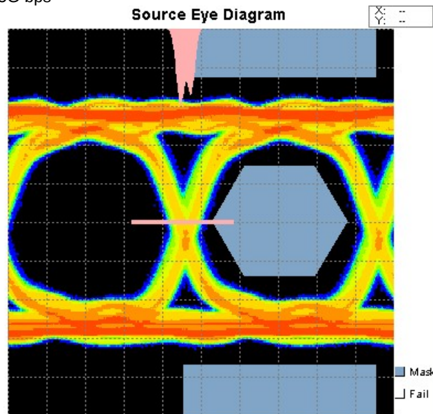
HDMI Port with MLSEP08A-2510
