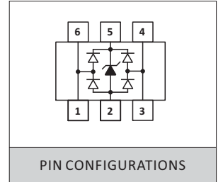
SOT-23-6 PACKAGE
